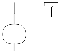
Kushi 33 suspension Ø 33 x H 56 Canopy Ø 12,5 x H 3
