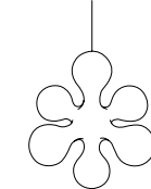
Atomium ceiling Ø 58 x H 52 Canopy Ø 12 x H 4,5
