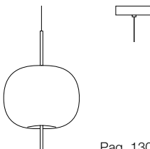
Kushi XL suspension Ø 43 x H 65 Canopy Ø 12,5 x H 3
